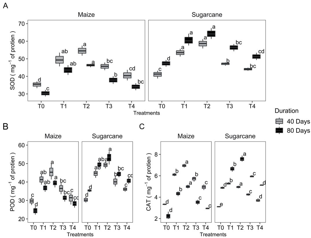
Fig. 2. Effect of metals contaminated dust on antioxidant activity of maize and sugarcane plants.
