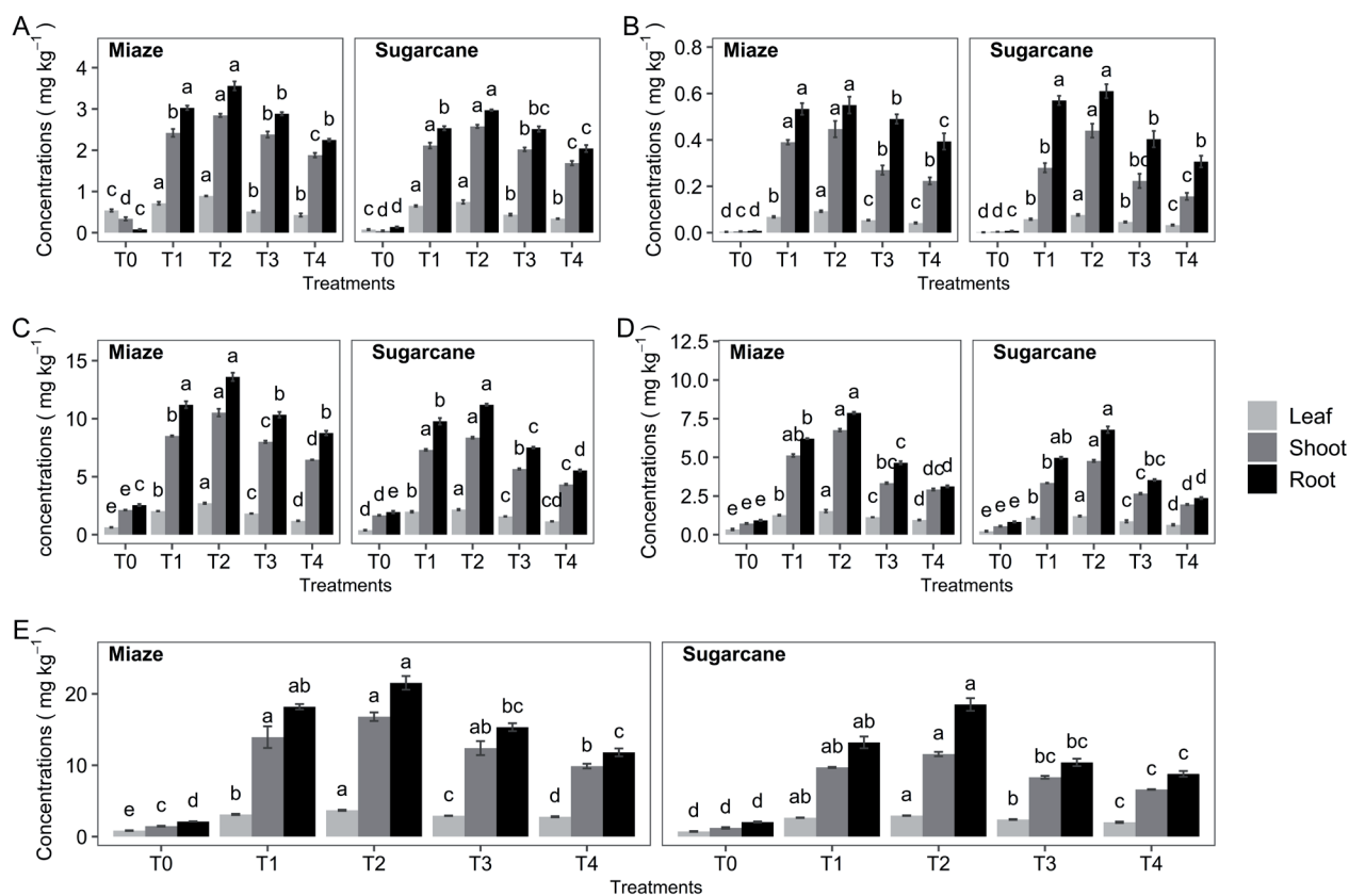
Fig. 3. Heavy metals concentrations in plant tissue of maize and sugarcane. Different letters represent significant difference among treatment ( p \leq 0.05 ); A = lead (Pb); B = cadmium (Cd); C = copper (Cu); D = nickel (Ni); E = zinc (Zn). All treatments were compared with the control (no dust) T0 = Control; T1 = 44-gram dust; T2 = 39-gram dust; T3 = 24-gram dust; T4 = 9-gram dust.
