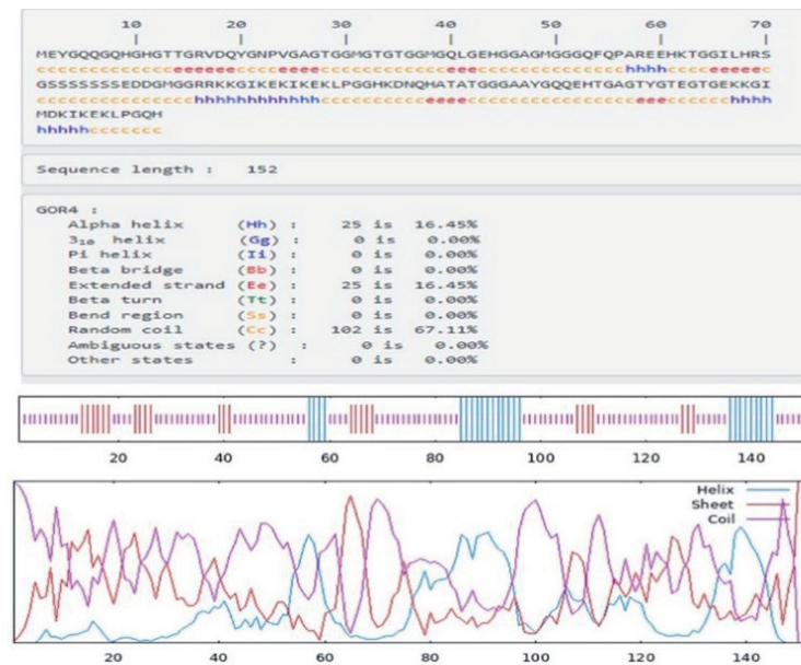
Fig. 3. The SbdHN1 protein's predicted secondary structure displays the length and location of the extended strands (e), random coils (c), and alpha helices (h).
