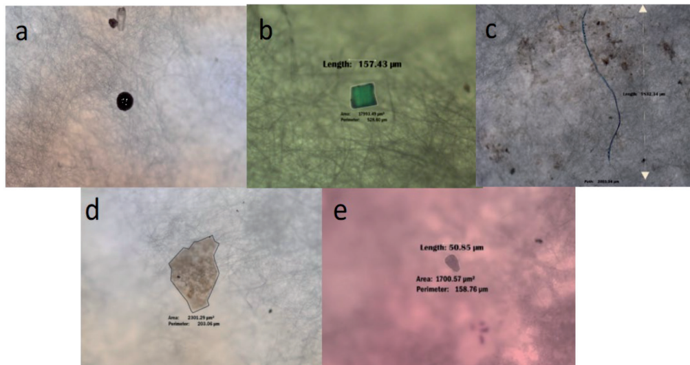
Fig. 4. Some microplastics found in the Opak River (a) pellet, (b) fragment, (c) fiber, (d) film, and (e) foam.
