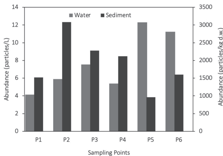
Fig. 2. The abundance of microplastics in the Opak river water and sediment.
