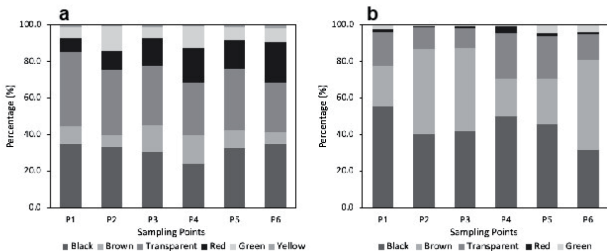
Fig. 5. Color of microplastic particles in Opak River (a) water and (b) sediment
