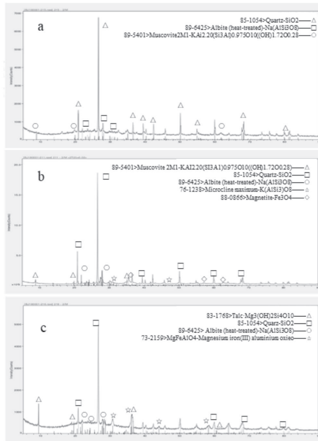
Fig. 5. XRD pattern result; (a: XRD pattern of the HM-contaminated soils; b: XRD pattern of the materials roasted beyond 800°C; c: XRD pattern of ceramsite).
