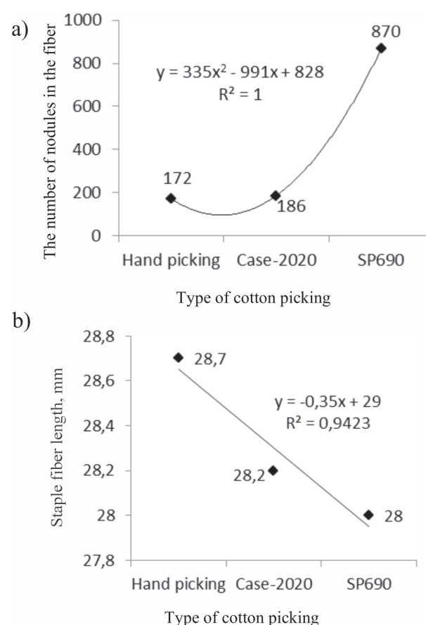
Fig. 2. Graphical analysis of the indicators of cotton fiber affecting spinning.
