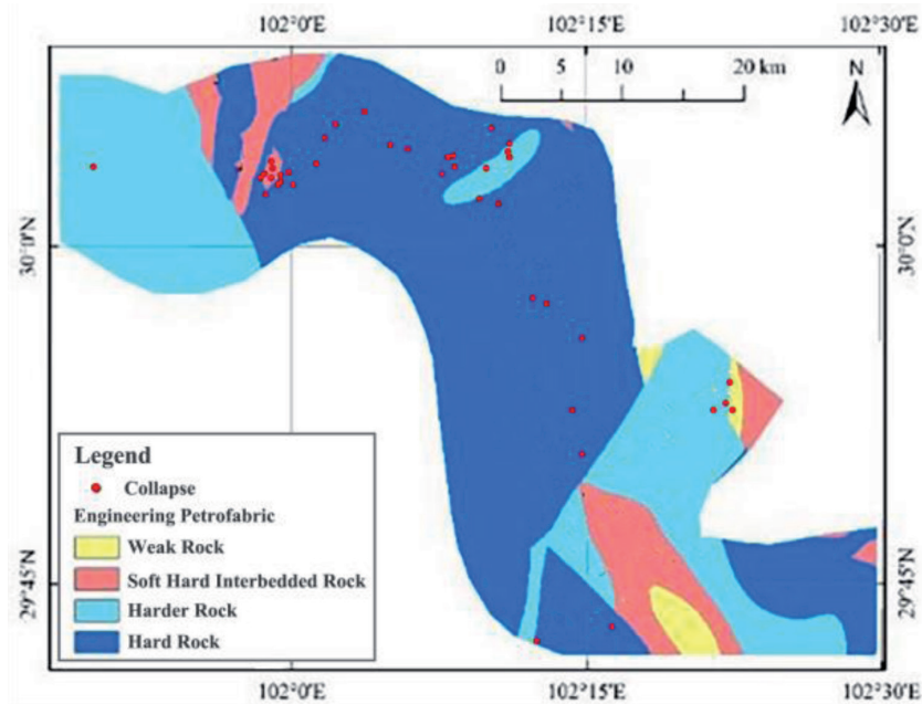
Fig. 5. The relation between the distribution of collapse disasters and rock formation
