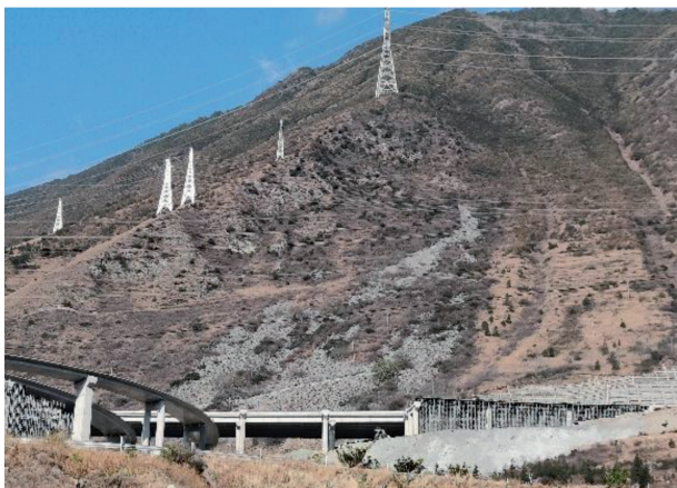
Fig. 7. Characteristics of No.4 collapse based on filed investigation
