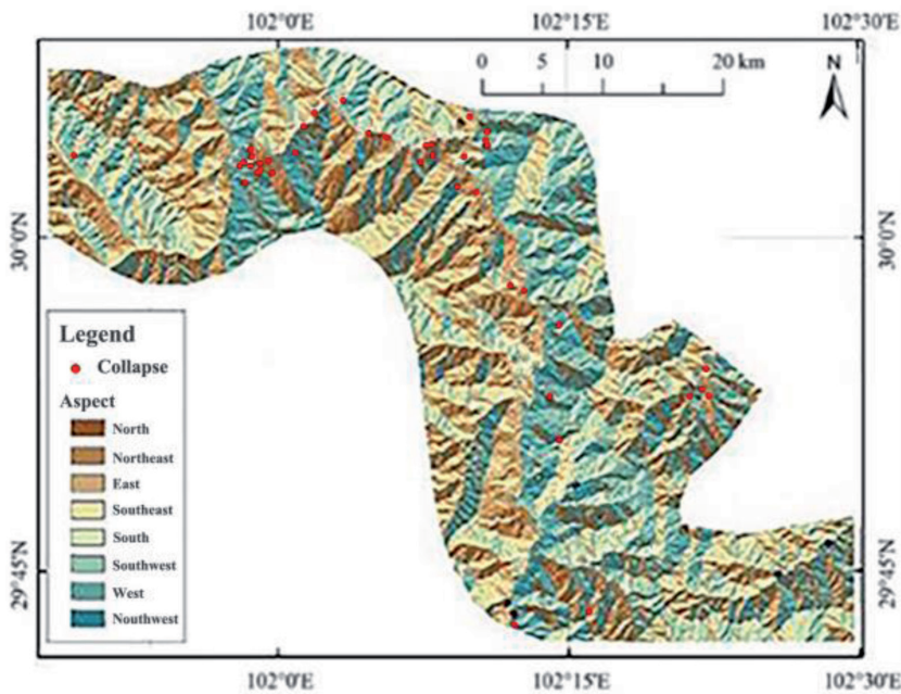
Fig. 3. The relation between the distribution of collapse disasters and slope orientation
