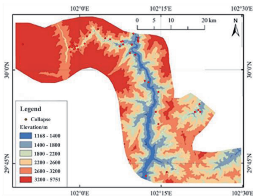
Fig. 1. The distribution map of geological disasters and elevation in the study area
