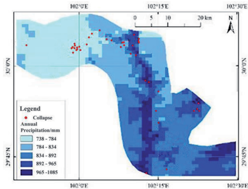
Fig. 6. The relation between the distribution of collapse disasters and annual rainfall
