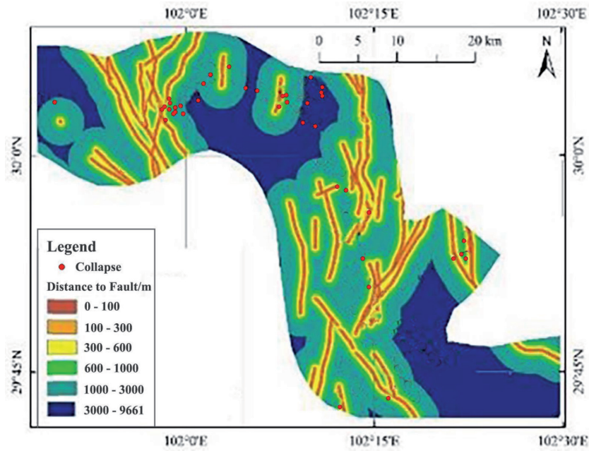
Fig. 4. The relation between the distribution of collapse disasters and distance from faults
