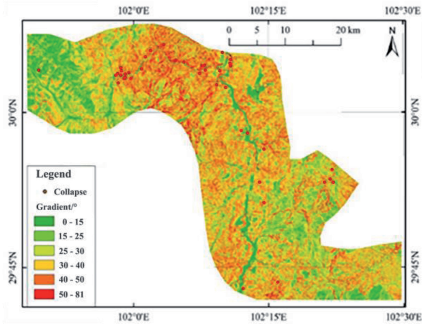
Fig. 2. The relation between the distribution of collapse disasters and slope gradient
