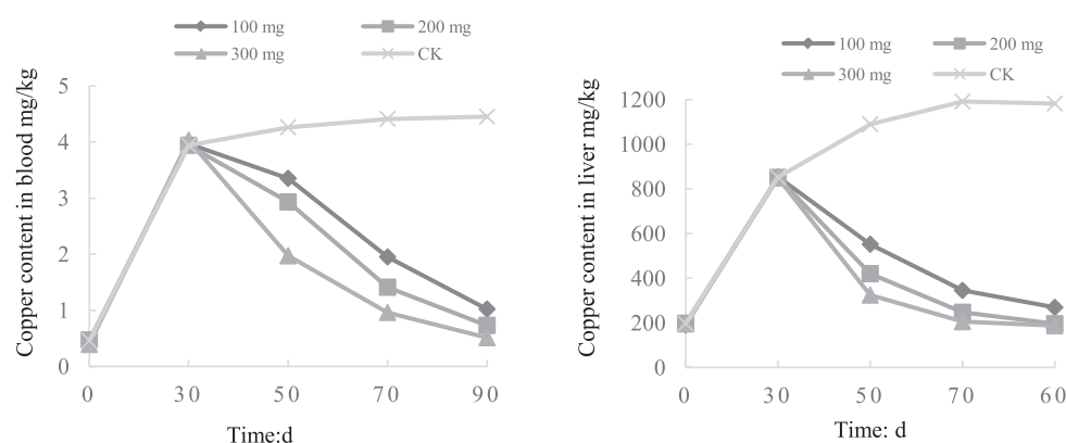
Fig. 1. Effect of ammonium molybdate on copper content in blood and liver.
